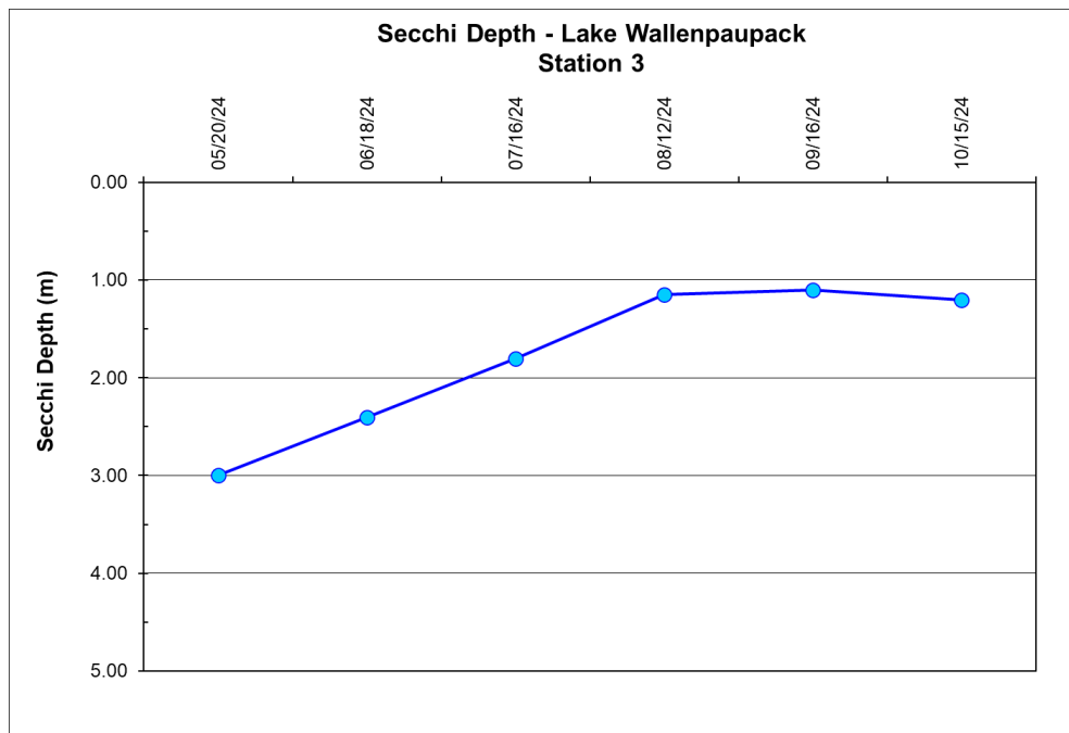
Figure 4.7 Secchi Disk Depths at Station 3 in 2024
