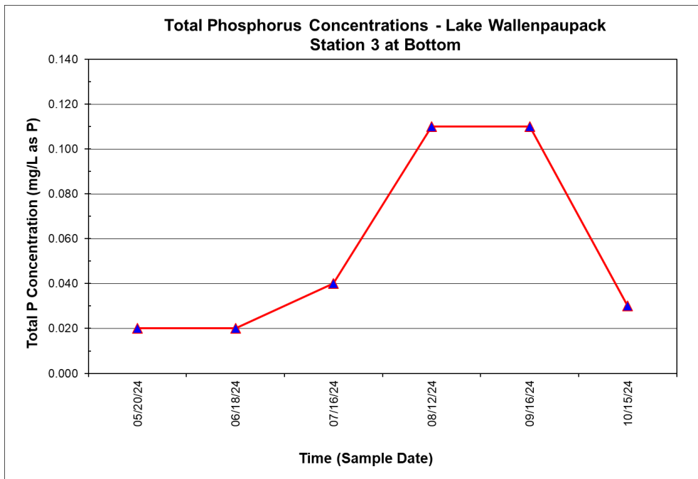
Figure 4.4 Total Phosphorus Concentrations at Station 3 Bottom in 2024
