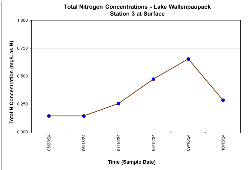
Figure 4.5 Total Nitrogen Concentrations at Station 3 Surface in 2024
