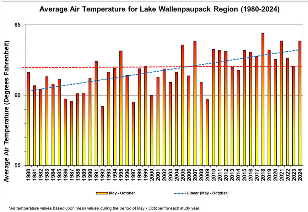
Figure 3.1 Historical Air Temperature Data in the Pocono Region
