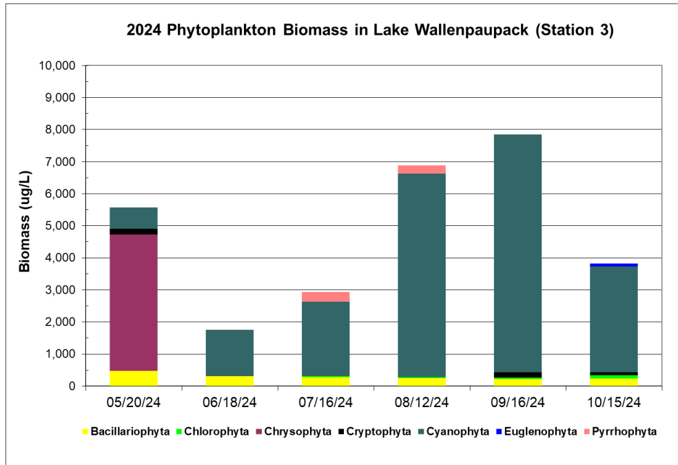
Figure 4.9 Phytoplankton Biomass at Station 3 in 2024
