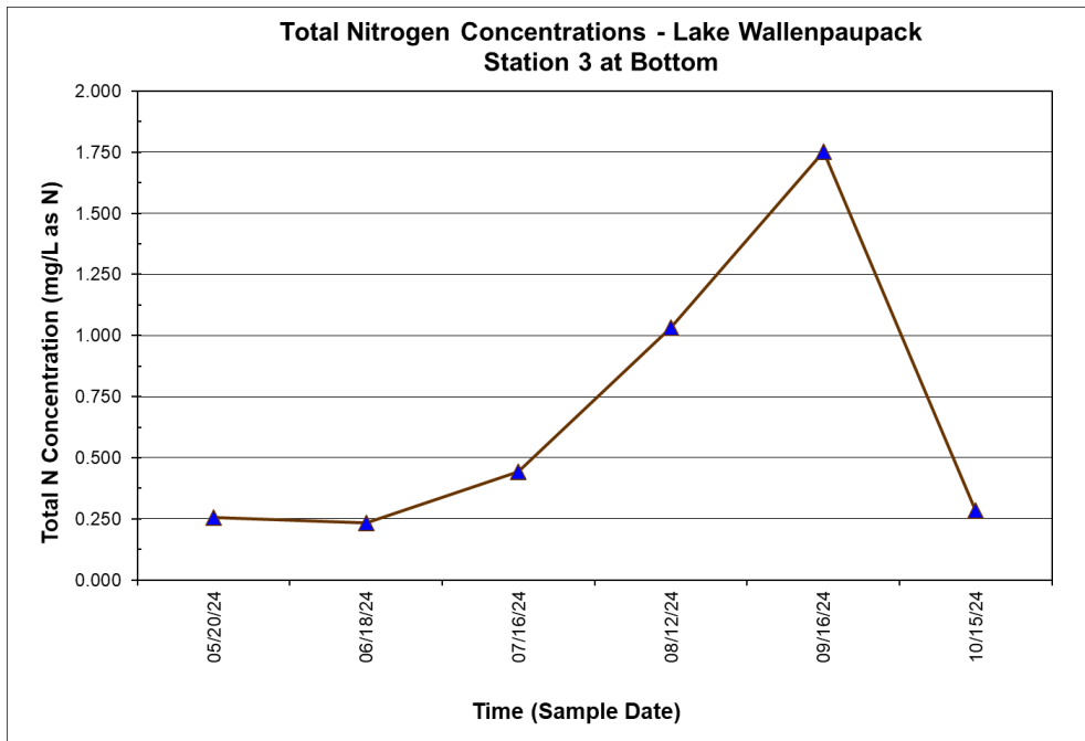
Figure 4.6 Total Nitrogen Concentrations at Station 3 Bottom in 2024
