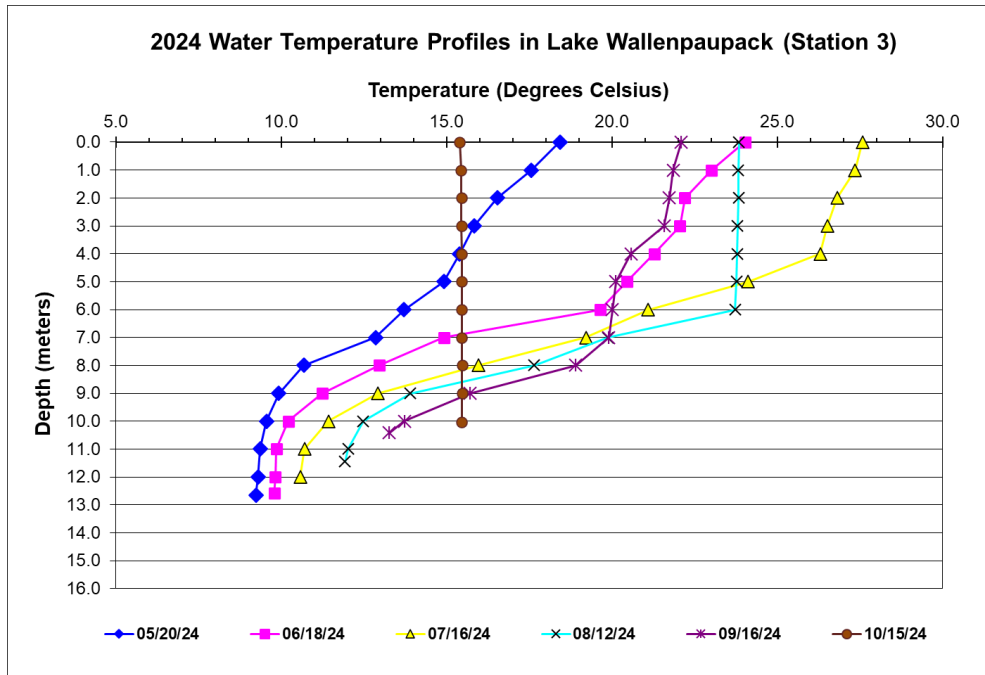
Figure 4.1 Water Temperature Profiles at Station 3 in 2024
