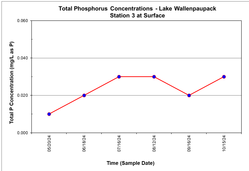
Figure 4.3 Total Phosphorus Concentrations at Station 3 Surface in 2024
