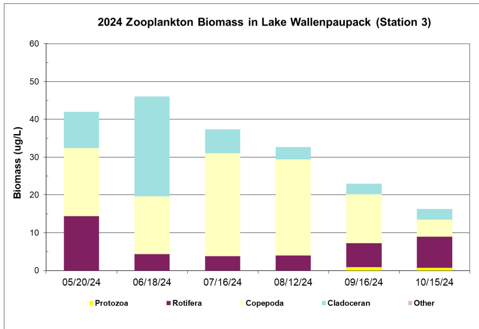
Figure 4.10 Zooplankton Biomass at Station 3 in 2024
