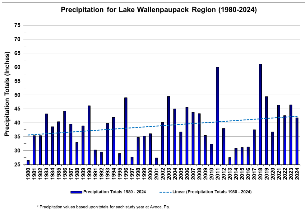
Figure 3.2 Historical Precipitation Data in the Pocono Region
