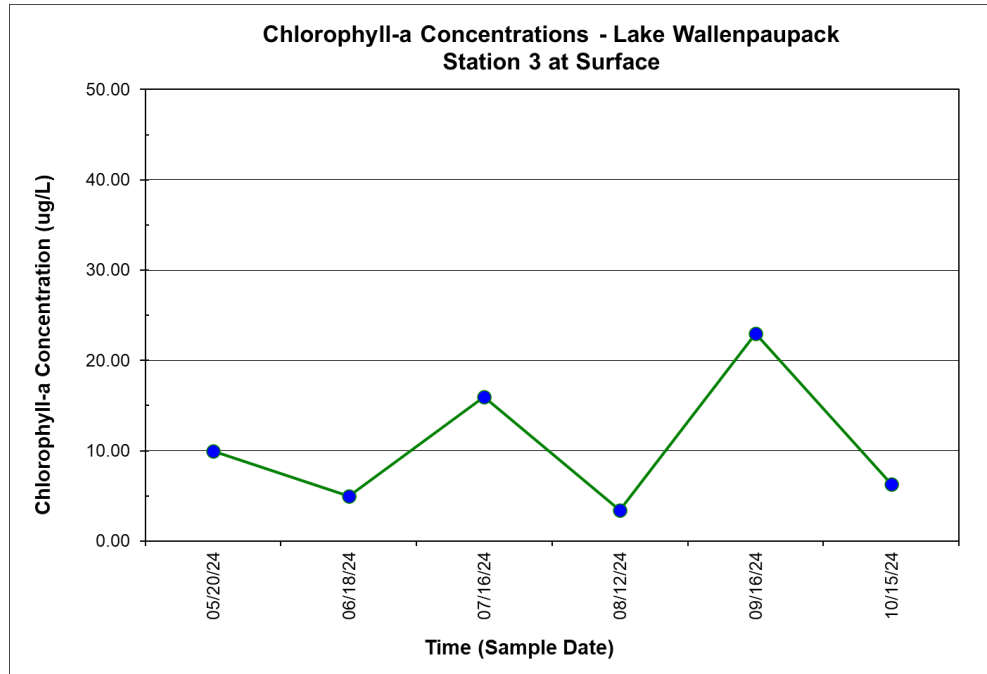
Figure 4.8 Chlorophyll-a Concentrations at Station 3 Surface in 2024
