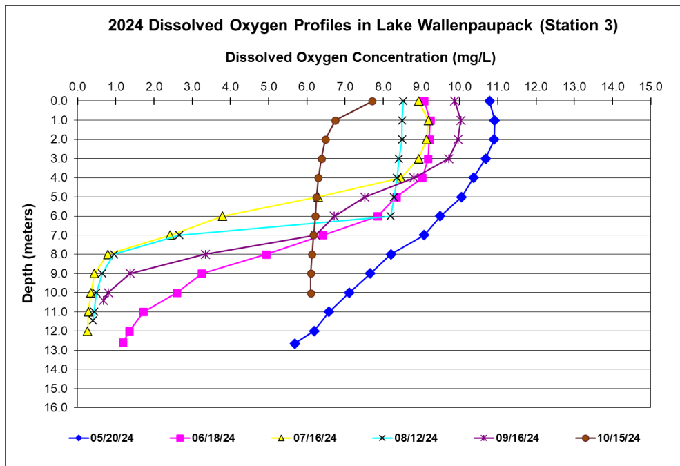
Figure 4.2 Dissolved Oxygen Profiles at Station 3 in 2024
