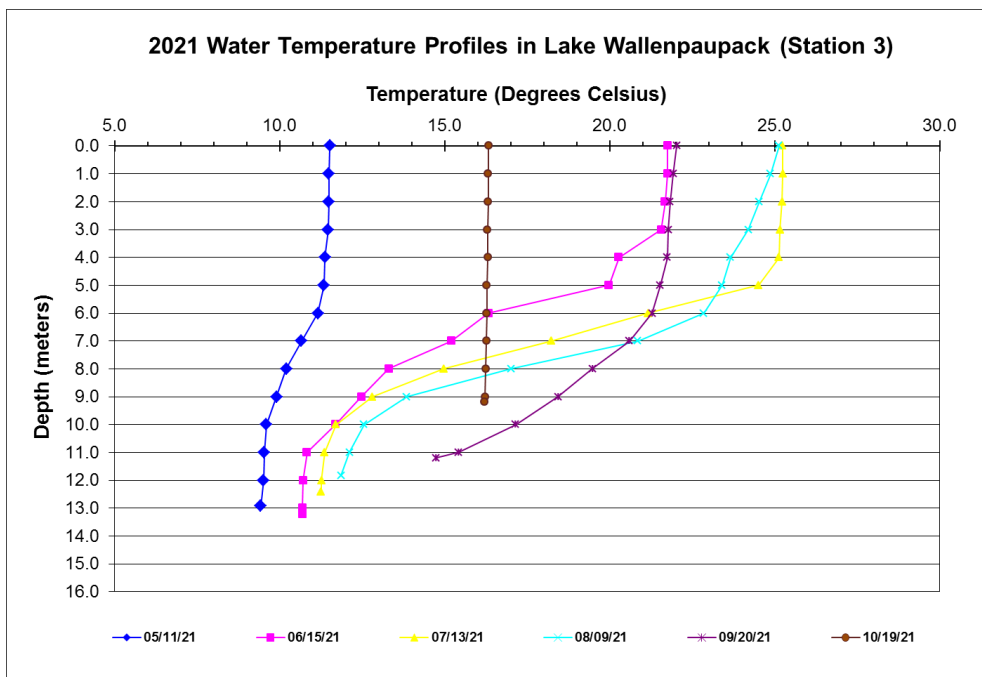
Figure 4.1 Water Temperature Profiles at Station 3 in 2021
