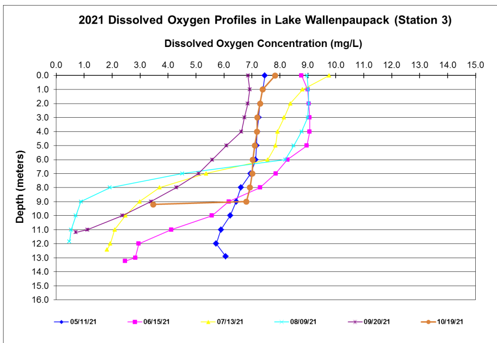
Figure 4.2 Dissolved Oxygen Profiles at Station 3 in 2021
