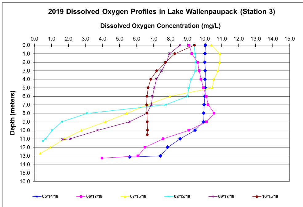
Figure 4.2 Dissolved Oxygen Profiles at Station 3 in 2019
