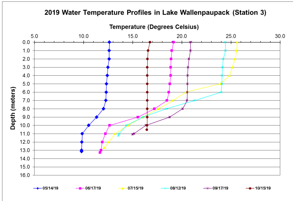
Figure 4.1 Water Temperature Profiles at Station 3 in 2019
