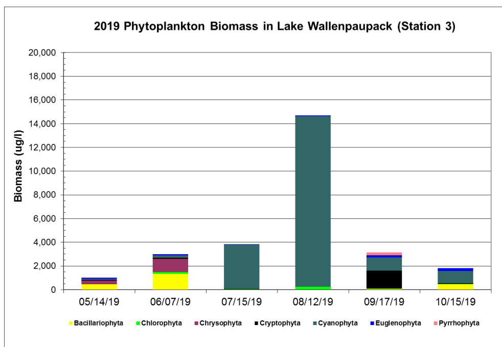
Figure 4.3 Phytoplankton Biomass at Station 3 in 2019
