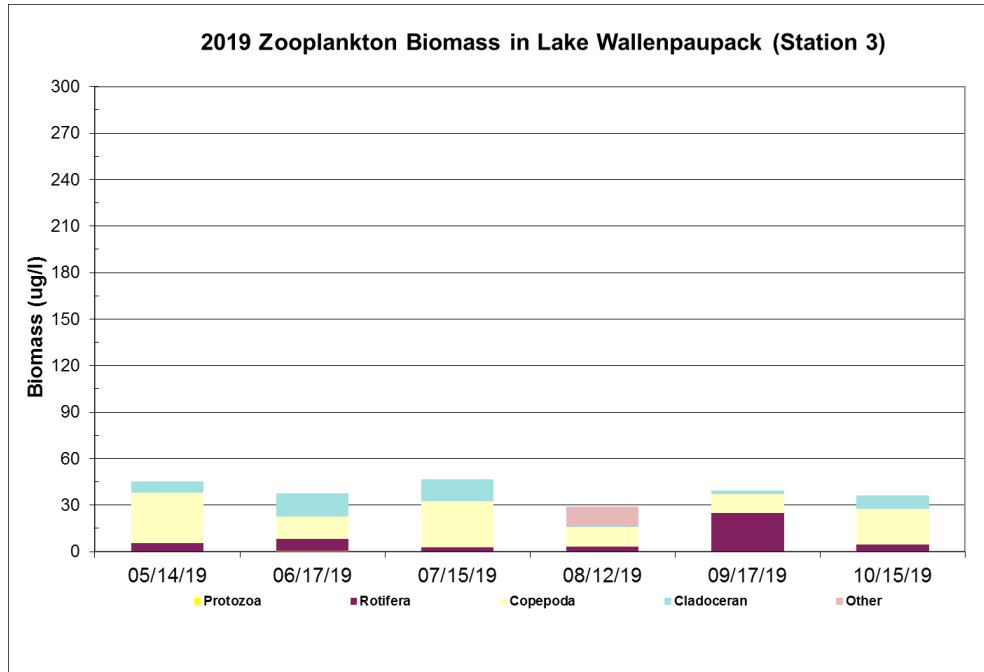
Figure 4.4 Zooplankton Biomass at Station 3 in 2019
